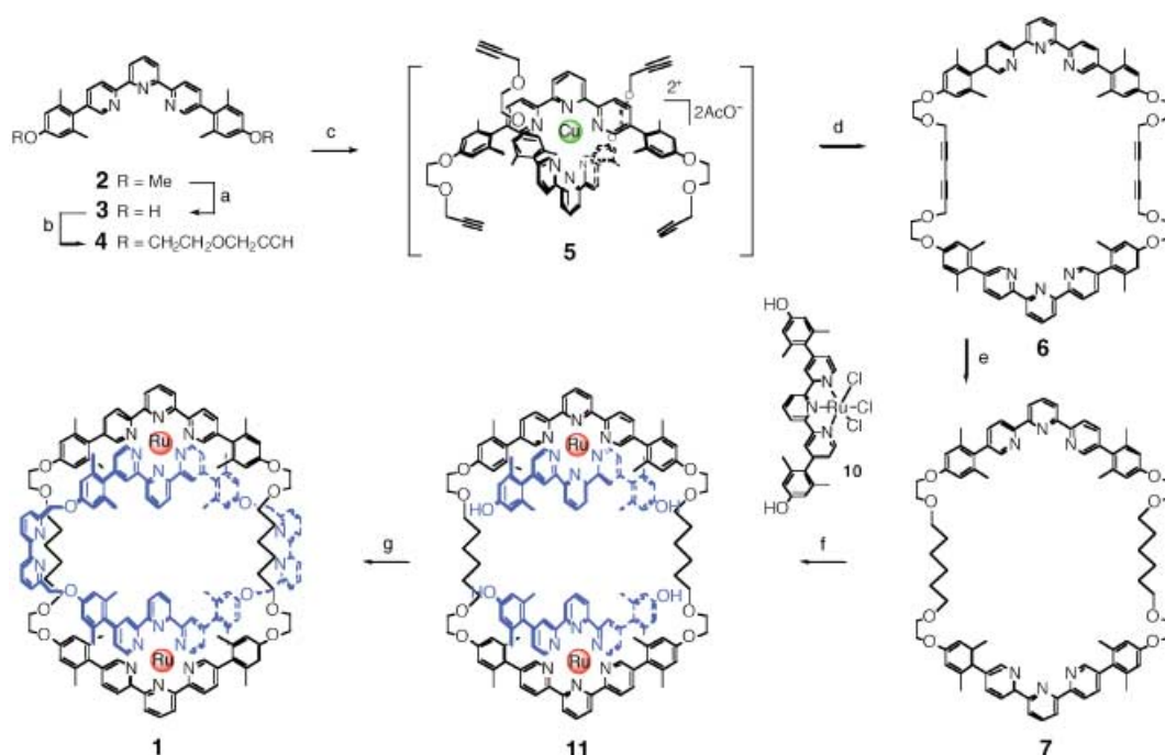
Scheme 1. Reaction conditions: a) molten py·HCl, 185 °C, 4 h, 97%; b) Cs 2 CO 3 , TsOCH 2 CH 2 OCH 2 CCH (2.2 equiv), DMF, 80 °C, 10 h, 69%; c) Cu(OAc) 2 ·H 2 O (0.5 equiv), ethanol, room temperature, 1 h; d) 1) Cu(OAc) 2 ·H 2 O (10.0 equiv), ethanol, high dilution, reflux, 72 h; 2) KCN (aq), CH 2 Cl 2 , 91%; e) H 2 80 psi, Pd/C (10%), ethanol/CH 2 Cl 2 (1:1), 6 h, 91%; f) 10 (2.0 equiv), CH 2 Cl 2 /EtOH/ethylene glycol (2:2:1), reflux, 12 h, 65%; g) 6,6'-bisbromomethyl-2,2'-bipyridine (2.0 equiv), Cs 2 CO 3 , acetonitrile, reflux, 72 h, 49%.
