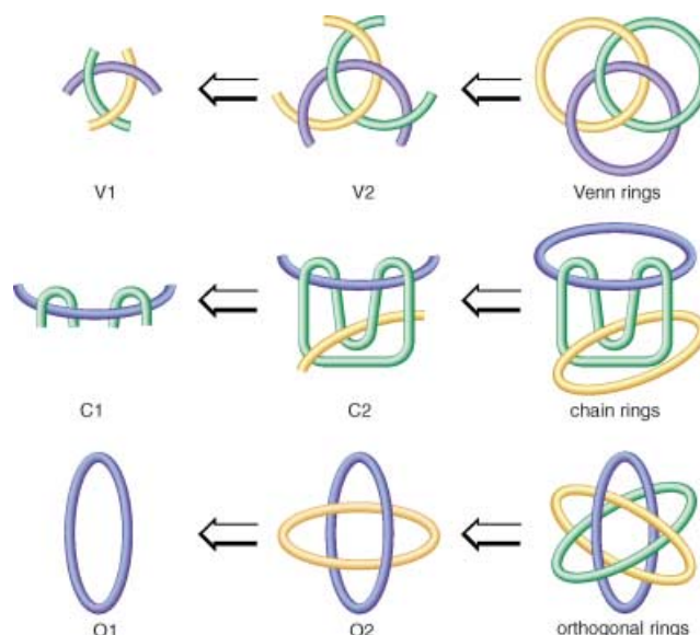
Figure 1. Three retrosynthetic representations of the Borromean link (Venn rings, chain rings, orthogonal rings).
