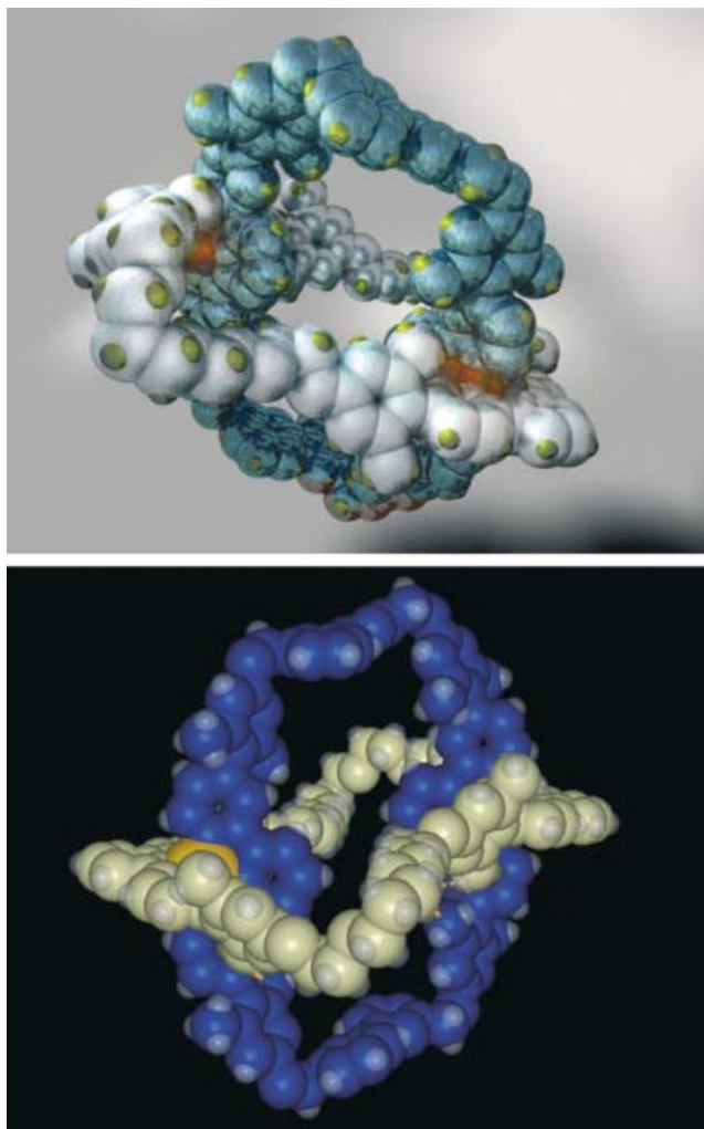
Figure 3. Space-filling model of the crystal structure of 1 : colored to emphasize connectivity; aspect to show chair form of ring 1 (bottom)
