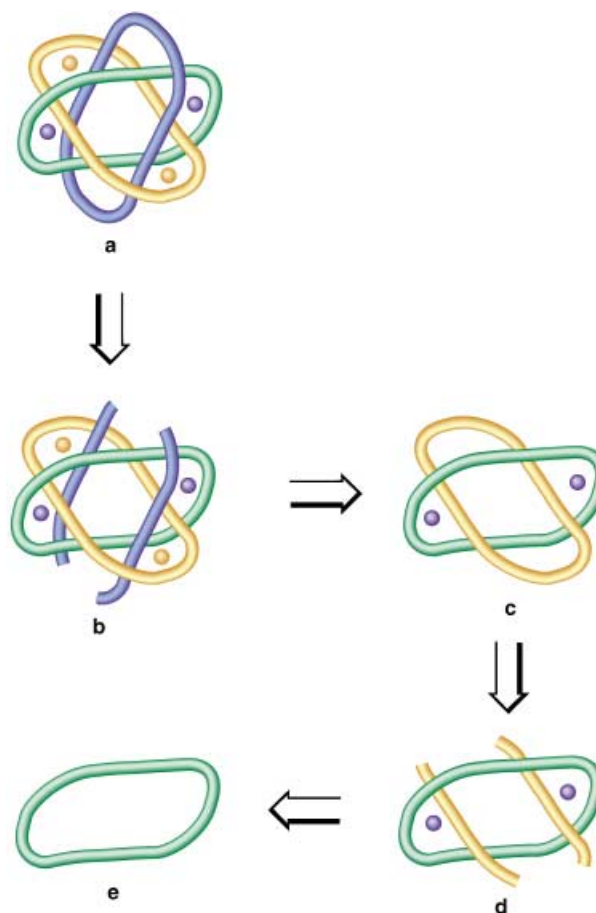
Figure 2. Retrosynthesis of a Borromean link from the orthogonal-ring representation.
